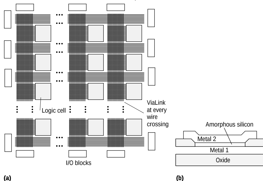
Figure 27. Quicklogic pASIC structure (a) and ViaLink (b).
