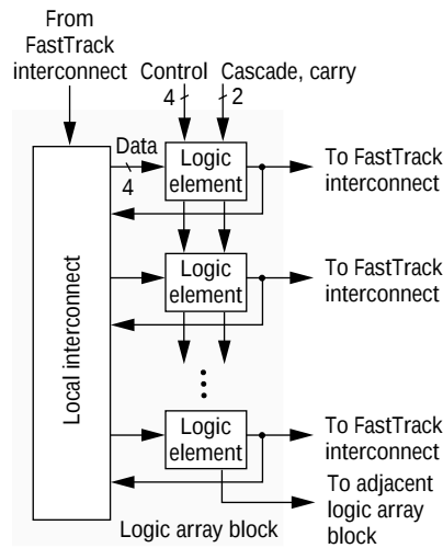
Figure 22. Flex 8000 logic array block.
