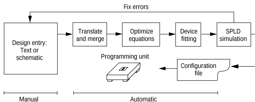
Figure 7. CAD process for SPLDs.
