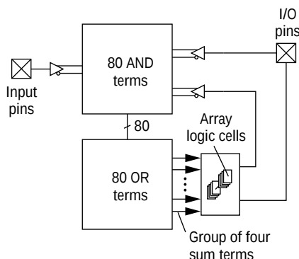
Figure 16. ICT PEEL Array architecture.
