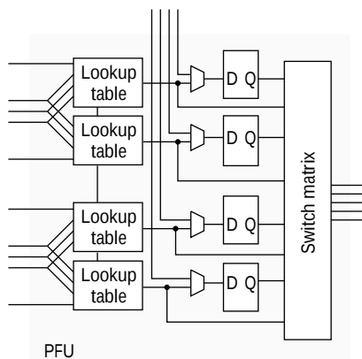
Figure 24. AT&T ORCA programmable-function unit.
