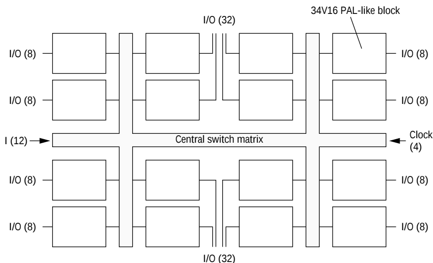
Figure 11. AMD Mach 4 structure.
