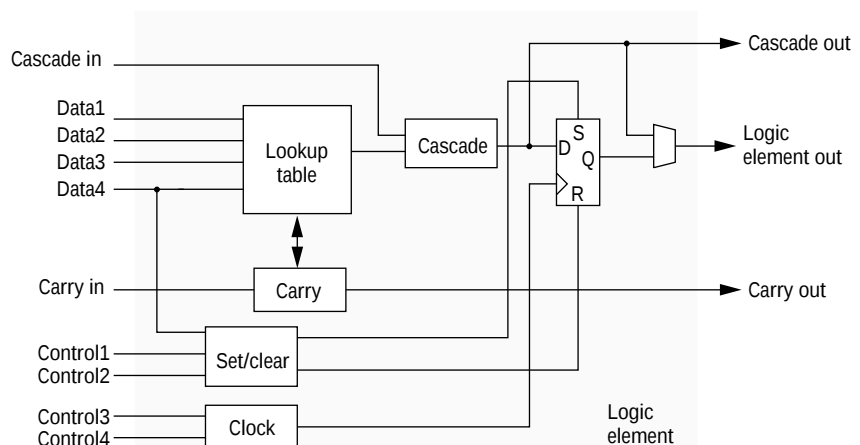
Figure 21. Flex 8000 logic element.
