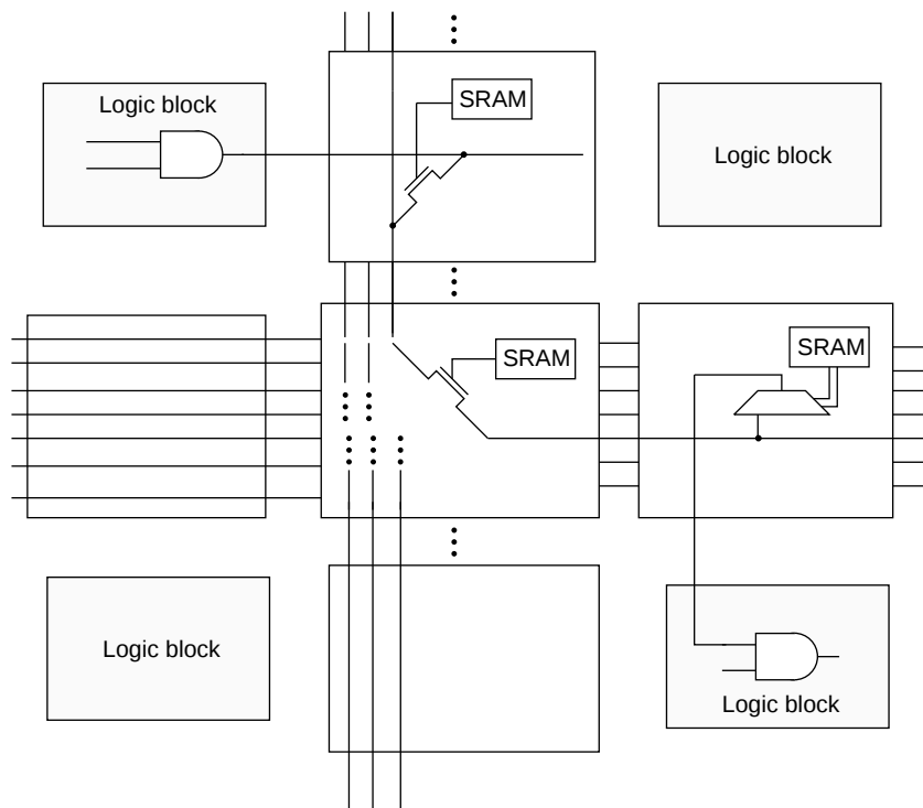
Figure 5. SRAM-controlled programmable switches.
