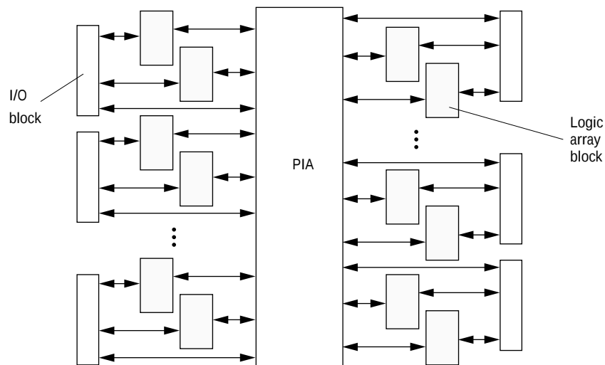
Figure 8. Altera Max 7000 series architecture.
