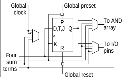
Figure 17. ICT PEEL Array logic cell structure.
