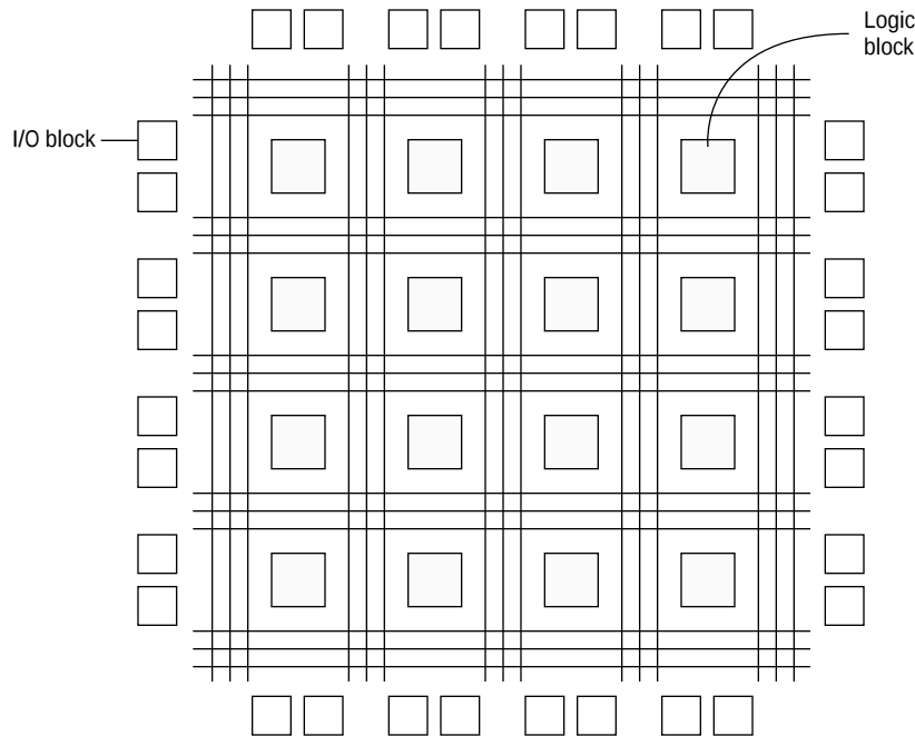
Figure 2. FPGA structure.
