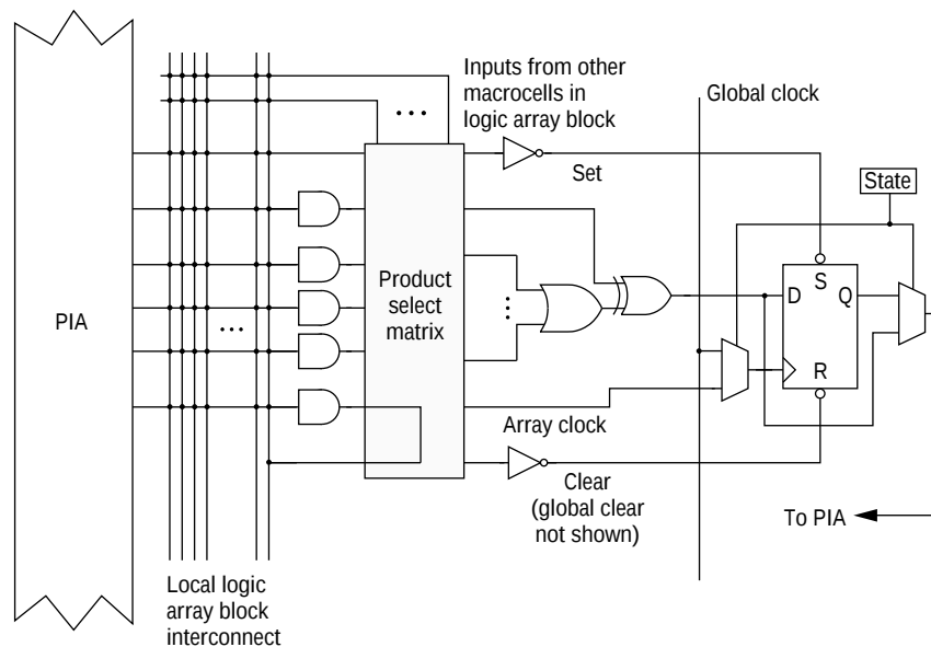
Figure 10. Max 7000 macrocell.
