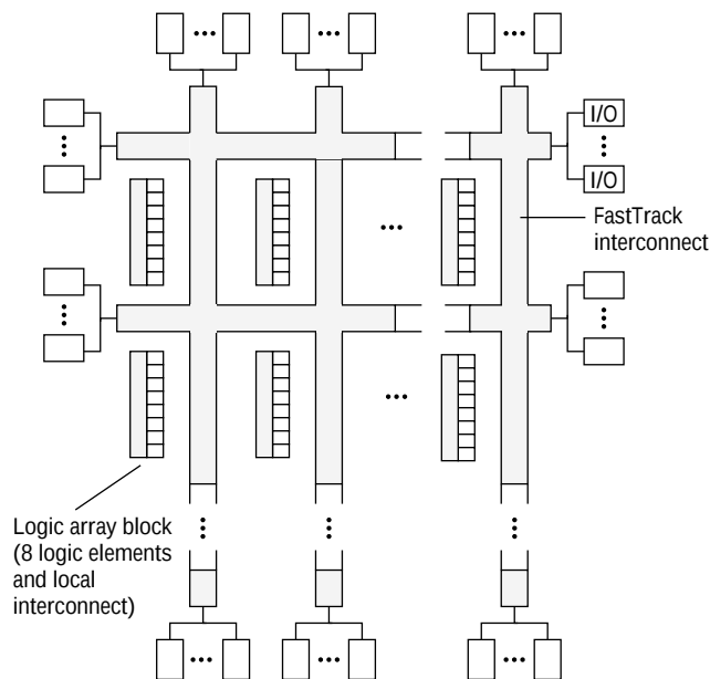
Figure 20. Altera Flex 8000 architecture.
