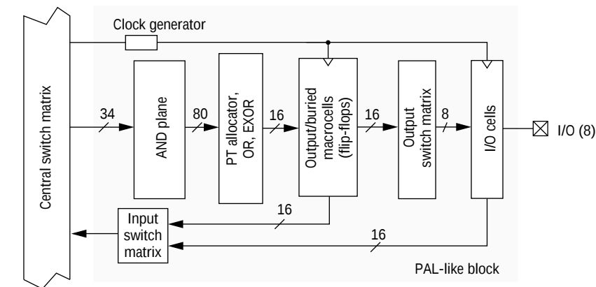
Figure 12. Mach 4 34V16 PAL-like block.
