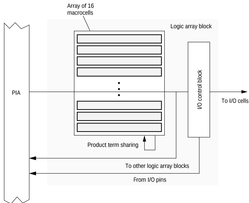
Figure 9. Altera Max 7000 logic array block.
