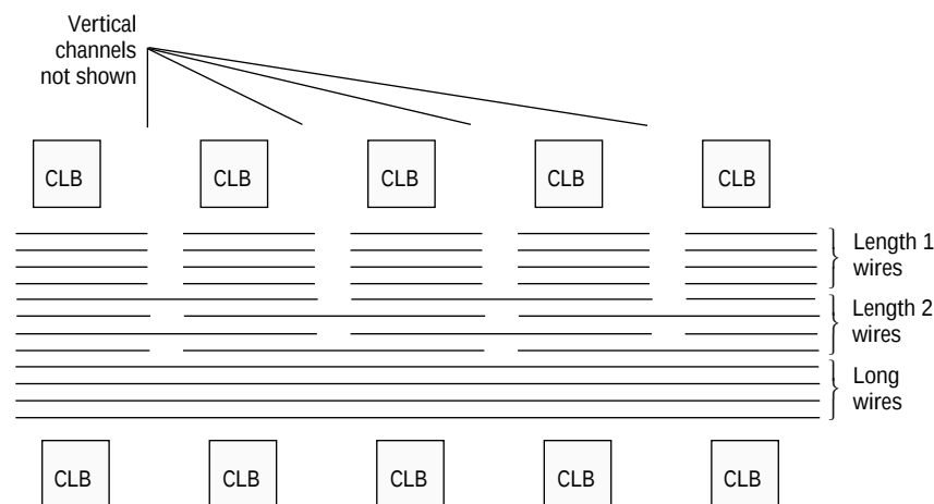
Figure 19. Xilinx XC4000 wire segments.
