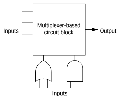
Figure 26. Actel Act 3 logic module.
