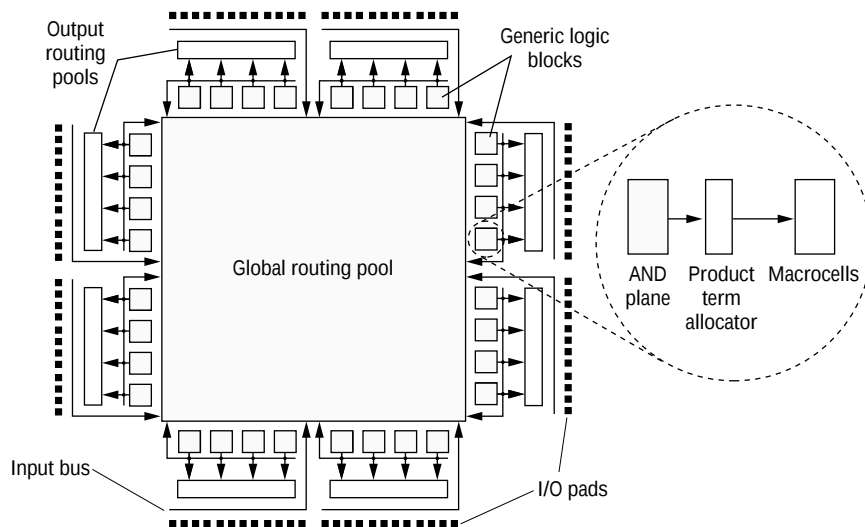
Figure 13. Lattice pLSI and ispLSI architecture.
