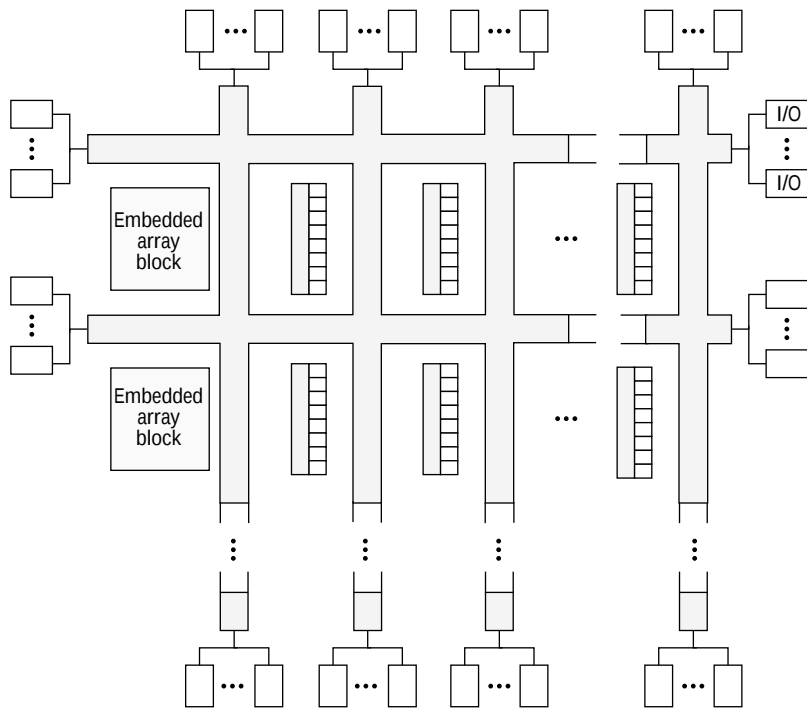
Figure 23. Altera Flex 10K architecture.
