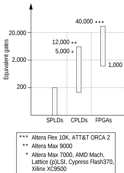
Figure 3. FPD logic capacities.
