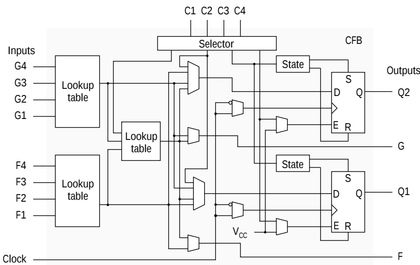
Figure 18. Xilinx XC4000 CLB.
