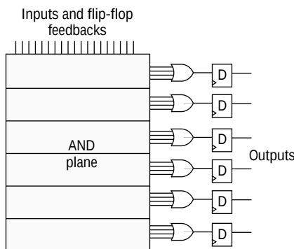
Figure 1. PAL structure.
