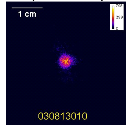
Effect of plasma plug and volume plasma on spot size
