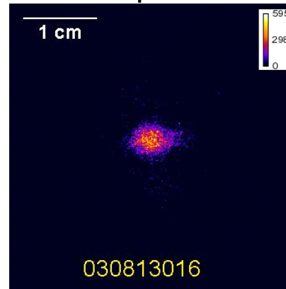
Effect of plasma plug on spot size
