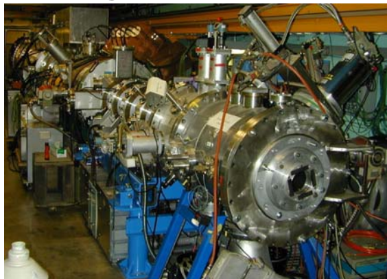
The HCX with magnetic quad section (2003)
