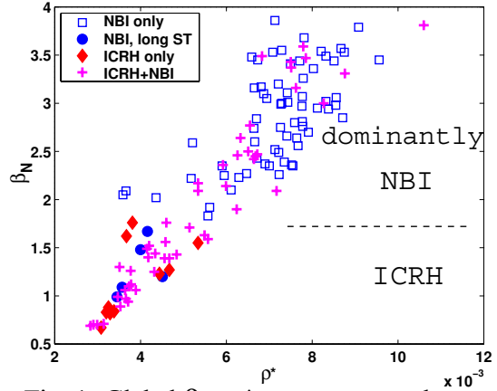
Fig. 1: Global \beta_N , \rho^* parameters at the onset of 3/2 modes for NBI and ICRH dominated discharges.
