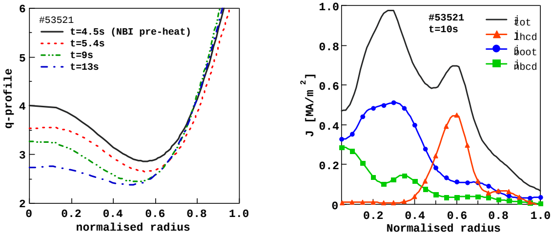
Fig. 3 : (left) q-profile evolution from polarimetry data (target q-profile at t = 4.5 \text{ s} in agreement with MSE data). (right) Non-inductive current profiles from TRANSP (#53521).
