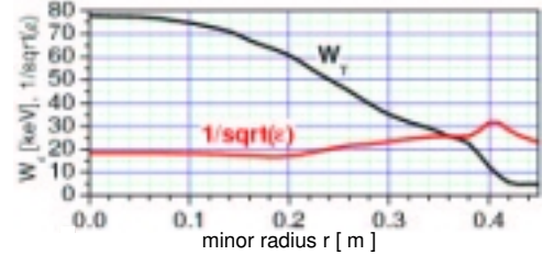
Figure 6. The lower energy limit W_\gamma for anisotropy effects due to E -field in discharge #14281.
