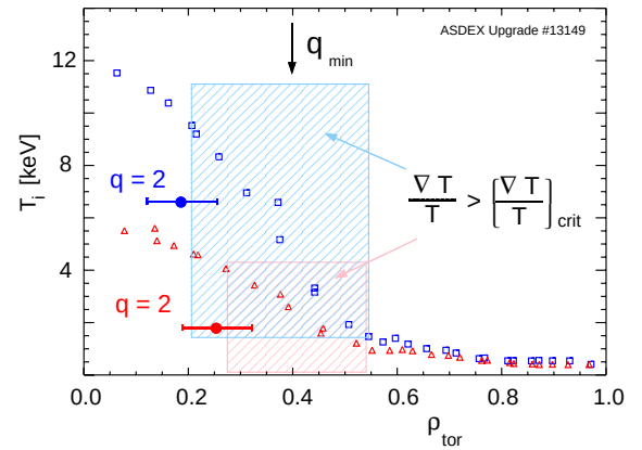
Fig. 2. Profiles of the ion temperature right after the onset of (2,1) fishbone activity ( t = 0.49 s) and just before the fishbone activity of (2,1) helicity disappears. In addition the location of the minimum q -value ( q_{\text{min}} ) and that of the inner q = 2 surface are given. Furthermore the radial extent of the ITB for the two times is shown by the hatched areas.
