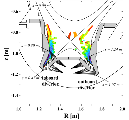
Figure 1: Simulated 465 nm C^{2+} emissivity [ \text{ph m}^{-3} \text{s}^{-1} \text{sr}^{-1} ] obtained from ‘DIVIMP’ and geometry of the measuring lines of sight in the divertor .
