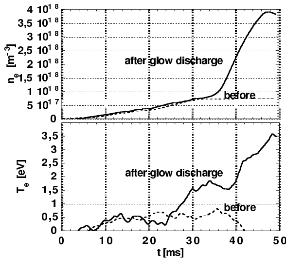
Fig. 4: Comparison of electron temperature and electron density of two pulses in W7-AS. One pulse was made before, the other one after discharge cleaning. The electron density and temperature rose very similarly during the first 30 ms. In the first case T_e decreased afterwards whereas it rose in the second case. The plasma ignited only after the walls were well conditioned. The neutral gas density in the vessel would be an important experimental parameter according to Fig. 3. It could not be measured, however.
