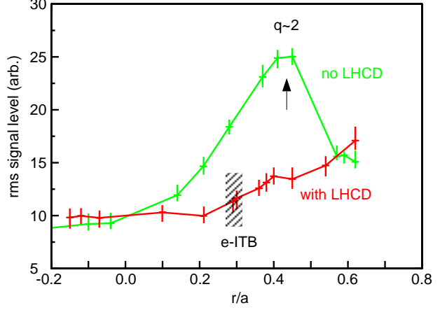
Figure 5: rms fluctuation level vs radius with (#53449) and without (#53453) LHCD.
