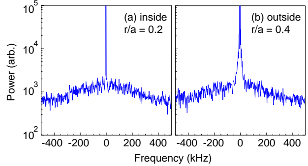
Figure 4: Reflectometer spectra: (a) inside e-ITB at t = 3.0 s, (b) outside e-ITB at t = 6.0 s; 96 GHz x-mode, shot #53449.
