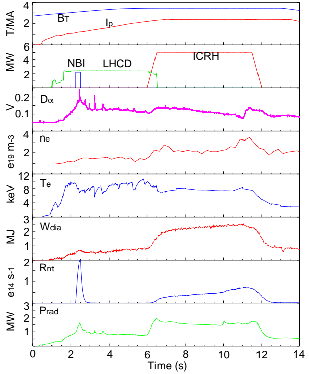
Figure 1: Plasma parameter time traces for 3.4T/2.6MA shot #53449.
