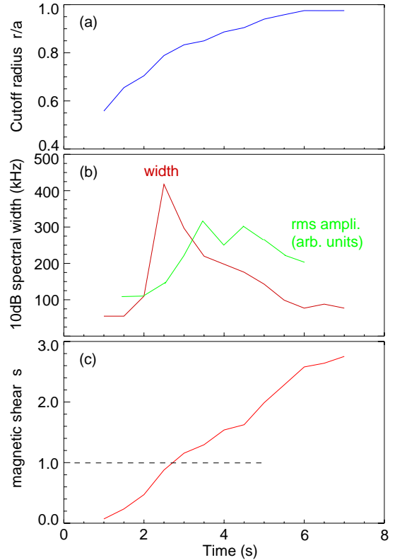
Figure 7: (a) 75 GHz x-mode cutoff, (b) spectral half-width & rms amplitude, (c) magnetic shear at cutoff, shot #52449.
