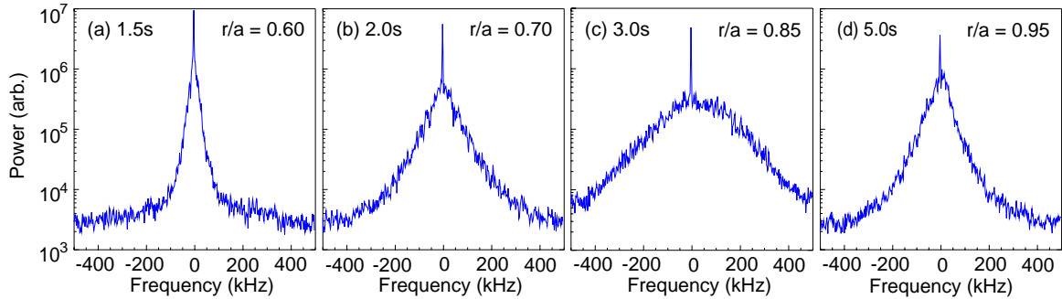
Figure 6: Complex amplitude spectra from 75 GHz x-mode edge channel #53453.
