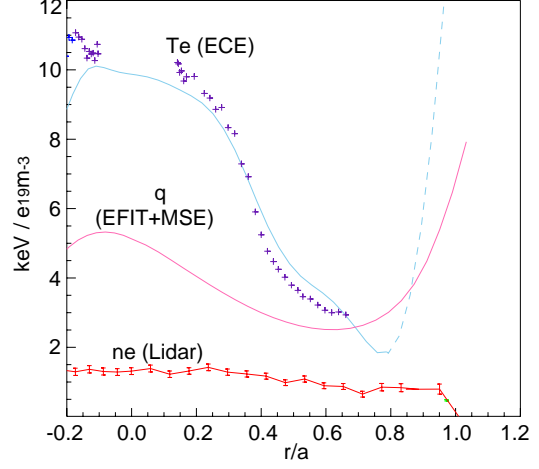
Figure 3: q , T_e , n_e profiles at t = 4.5 s in LHCD + ICRH shot #53557.
