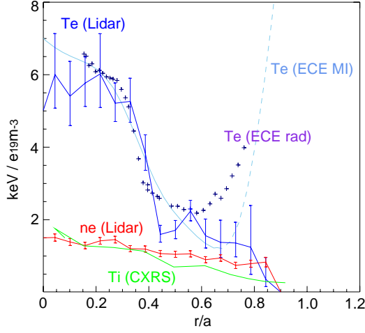
Figure 2: T_e (ECE, Lidar), T_i (CXRS), n_e (Lidar) profiles, t = 2.8 s in #53449.
