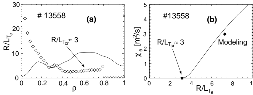
Fig. 5 (a) Critical (points) and experimental (line) R/L_{T_e} profiles. (b) \chi_e dependence on R/L_{T_e} from the Weiland model (other parameters from experiment at \rho = 0.63 ); modeled \chi_e and R/L_{T_e} at \rho = 0.63 (diamond).
