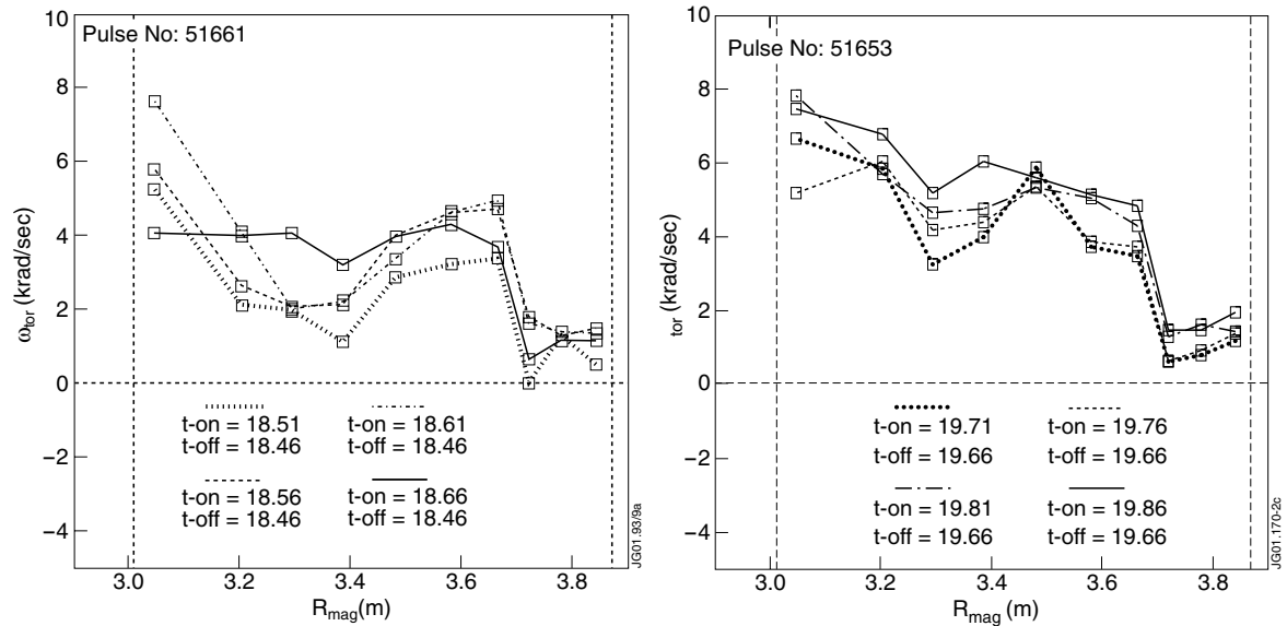
Figure 2. On the left (a), rotation profile for a location of the resonance layer at R = 2.5 m, P_{\text{IC}} = 2.85 MW, on the right (b) for a location of the resonance layer at R = 2.65 m, P_{\text{IC}} = 2.9 MW. In both cases the plasma was in the L-mode. Four rotation profiles taken during a time interval of 200 ms are shown. As discussed in the text, the first profile is not markedly influenced by the momentum input of the beam.
