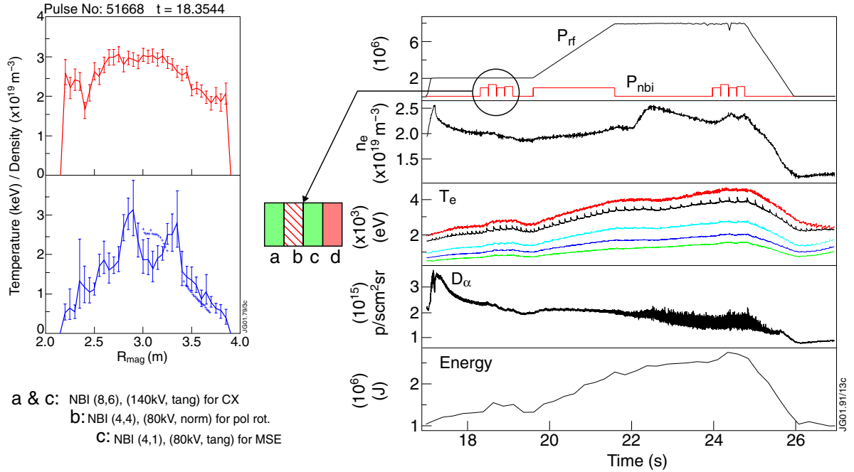
Figure 1. On the right, typical time traces of ICRF and NI power, plasma density and temperature, D_\alpha signal and plasma energy. In the sequence of beam blips, the first and third (a and c) in each series of 4 blips, is used to measure the toroidal rotation. On the left, profiles of the density (top) and of the temperature (bottom).
