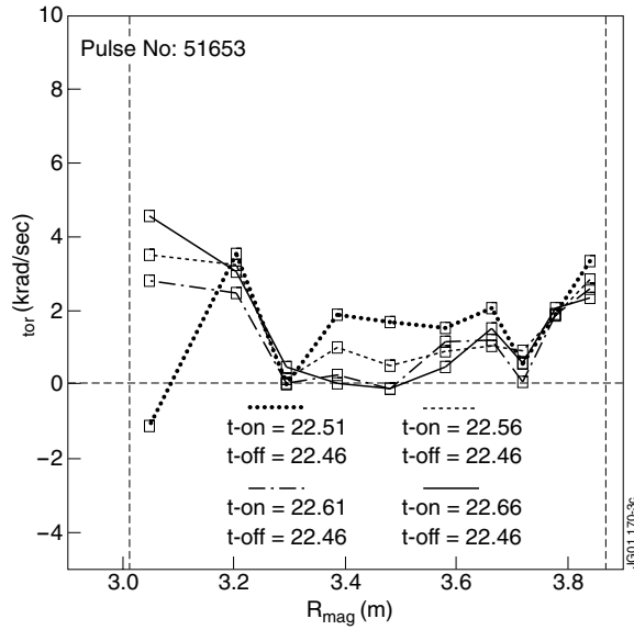
Figure 3. Toroidal rotation profile for the same discharge as fig 2b, at a later time, R = 2.95 m, P_{IC} = 2.9 MW, after a period of sawtooth stabilization and subsequent large sawtooth crash.
