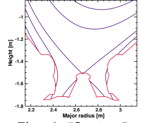
Fig. 1 "Septum" configuration: the X-point is lying on the dome of the MkIIIGB divertor
