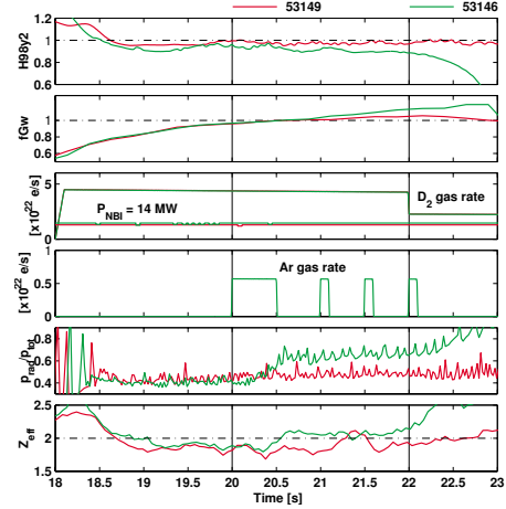
Fig. 5 Time traces of global plasma parameters for two discharges: unseeded reference (red) and with impurity seeding (green): confinement enhancement factor, Greenwald fraction, beam power and D_2 gas rate, Ar gas rate, total radiated power and Z_{eff} .
