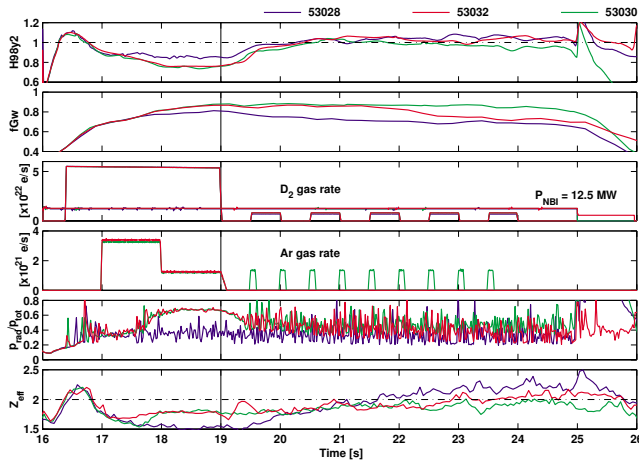
Fig. 2 Time traces of global plasma parameters for three discharges: unseeded reference (blue), with impurity seeding in the "puff" (red) and with impurity seeding both in the "puff" and in the "afterpuff" (green): confinement enhancement factor, Greenwald fraction, beam power and D_2 gas rate, Ar gas rate, total radiated power fraction and Z_{eff}
