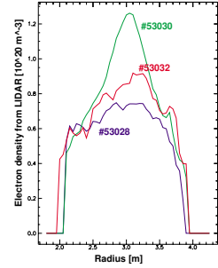
Fig. 3 Density peaking for the three shots of fig. 2 taken at 22.9 s.
