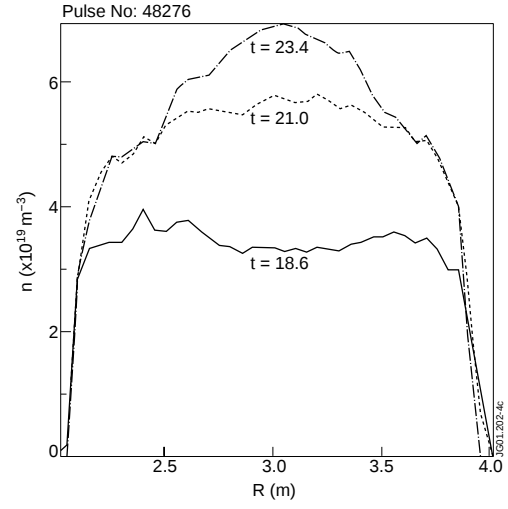
Fig. 3. The electron density profile at three times.
