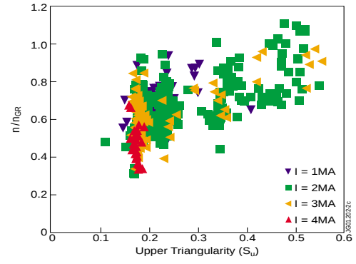
Fig. 4. n/n_{GR} versus the upper triangularity \delta_u , current grouping as in Fig. 1
