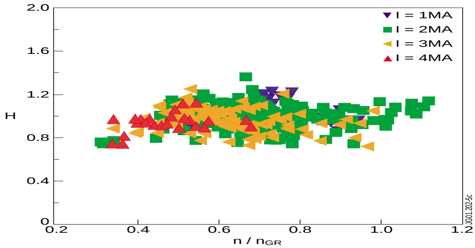
Fig. 5. The fit for the H factor given by Eq. (4) versus n/n_{GR} .
