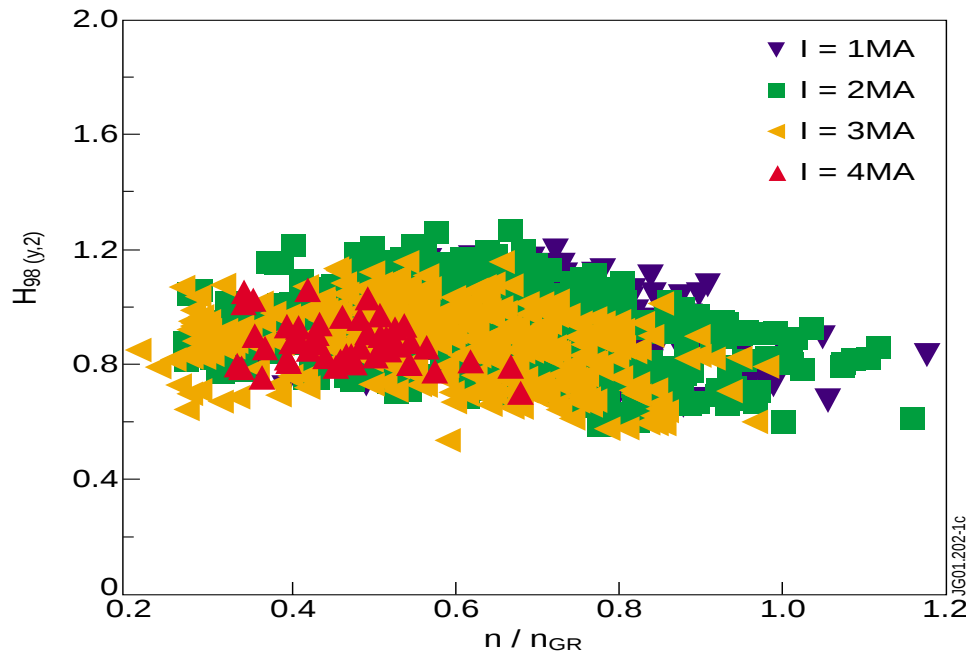
Fig. 1. H_{98} (\equiv \tau_{th}/\tau_{E98}) versus n/n_{GR} , the data are grouped by current I in MA 0.5 < I < 1.5 , 1.5 < I < 2.5 , 2.5 < I < 3.5 and I > 3.5 .
