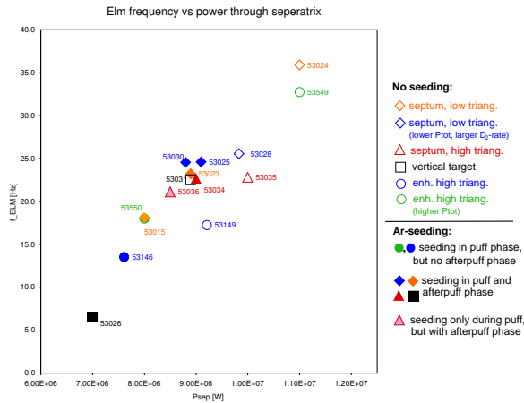
Fig. 4: ELM frequency versus power crossing the separatrix. The open symbols correspond to unseeded pulses, the closed to seeded.
