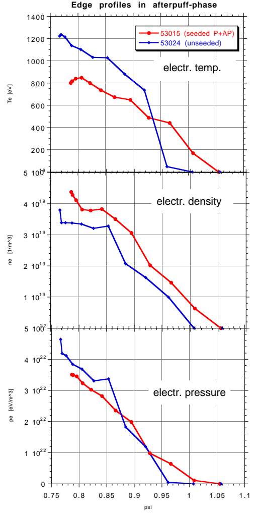
Fig 3: Edge profiles of seeded and unseeded pulse. The profiles are taken during the afterpuff phase at the time as indicated in Fig. 1.
