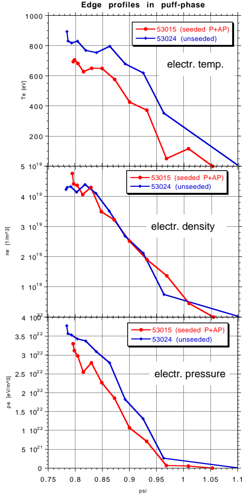
Fig 2: Edge profiles of seeded and unseeded pulse. The profiles are taken during the puff at the time as indicated in Fig. 1.
