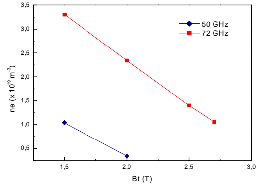
Fig 2 - Higher density values for the magnetic fields considered in Fig. 1 and a given density profile with n_{e0} = 7 \times 10^{19} \text{ m}^{-3} ; \alpha = 7 ; \beta = 1
