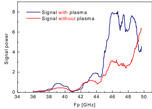
Fig 4 – Signal power from the two signals showed in Fig 3 with and without plasma
