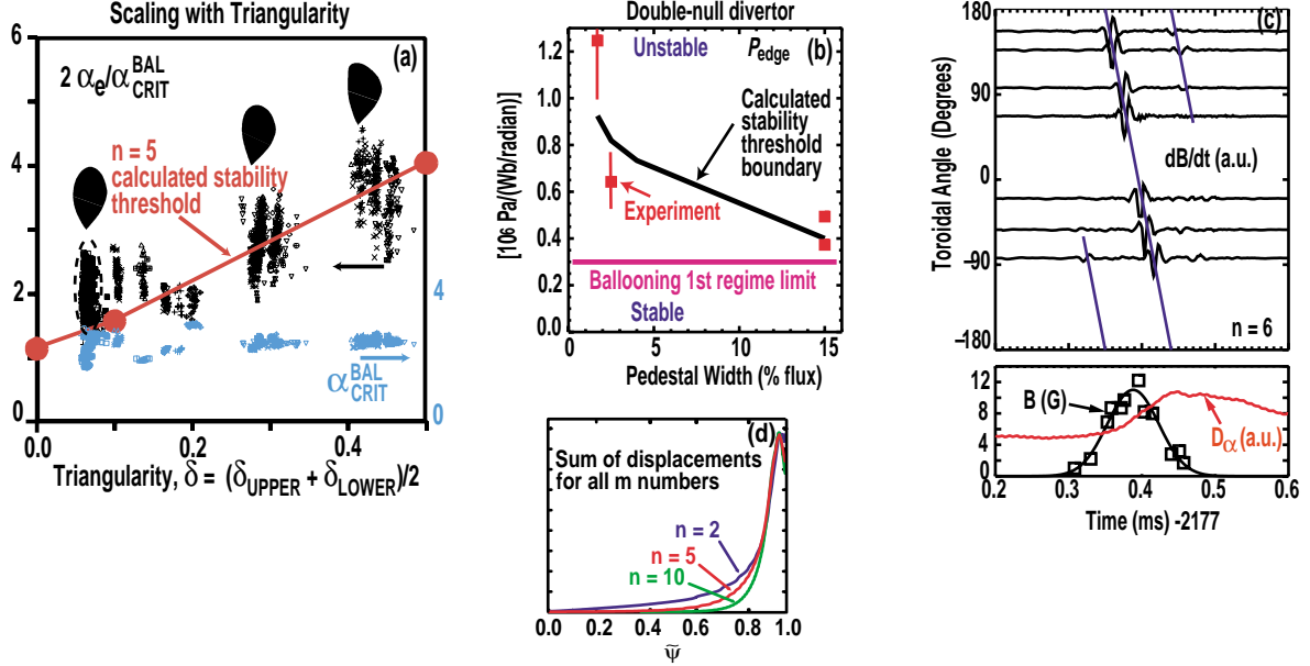
Fig. 1. (a) Edge pressure gradient before Type I ELM normalized to ideal ballooning mode limit increases with triangularity in agreement with ideal low n kink/ballooning mode calculation. Circled points correspond to variation in transport barrier width. (b) Critical edge pressure gradient for n=5 mode decreases with increasing width of the steep gradient region. (c) Fast growing low n modes observed as precursor to Type I ELM. (d) Radial modes structure of low n edge kink/ballooning mode.
