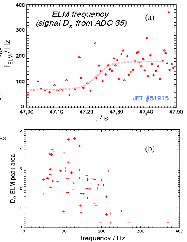
Fig. 2: (a) changes of the ELM-frequency. (b) area of ELM peak decreases with frequency.
