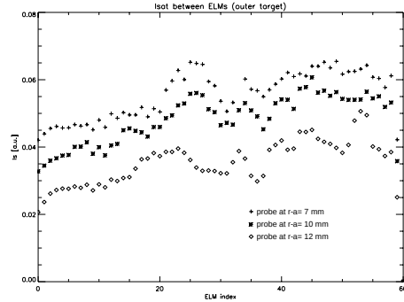
Fig. 5: Ion saturation current in between ELMs of three probes at the outer target is increasing in time.
