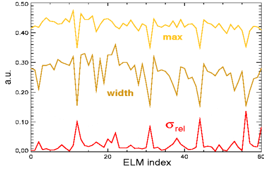
Fig. 3: Peak maximum, peak width and standard deviation of each ELMs. The four spikes in \sigma_{rel} occur on a regular time pattern.
