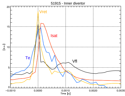
Fig. 6: Ion saturation current, floating potential, return voltage and electron temperature of average ELM. The peak of I_{sat} is delayed.
