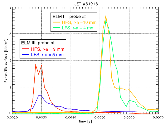
Fig. 7: Electron power flow of averaged type III ELMs ( t=47-47.5 ) and during type I ELMs ( t=48.8-49.2 ). The type I are plotted with an arbitrary time offset.
