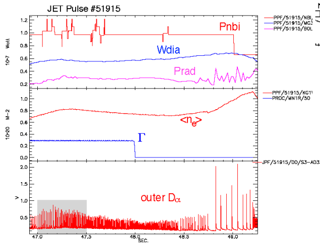
Fig. 1: Time traces of neutral beam power, plasma diamagnetic energy, radiated power, line integrated central density, gas flow \Gamma and recycling at the outer divertor box ( D_\alpha ). The grey shaded box indicates the series of analysed ELM
