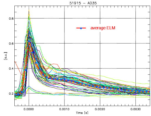
Fig. 4: All individual ELMs and the resulting average ELM. Note the four small exceptional ELM-events.
