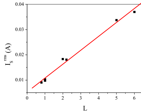
Fig. 3: The scaling factor versus the RMS of ion saturation current
