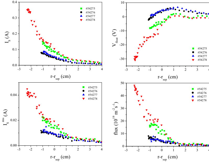
Fig. 1: Radial profiles of ion saturation current , floating potential, RMS of ion saturation current and ExB turbulent transport with different plasma densities.
