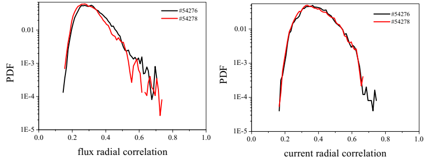
Fig. 4: PDF's of the radial coherence of ExB transport and ion saturation current fluctuations.
