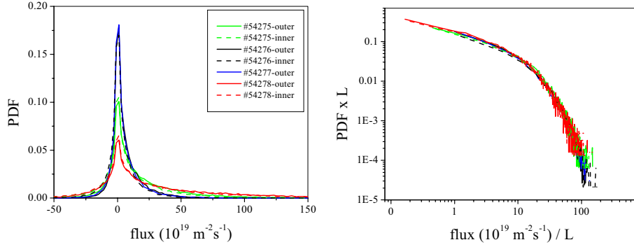
Fig. 2: Probability distribution function of ExB turbulent fluxes for different plasma densities measured in the plasma edge region and re-scaled PDF's.
