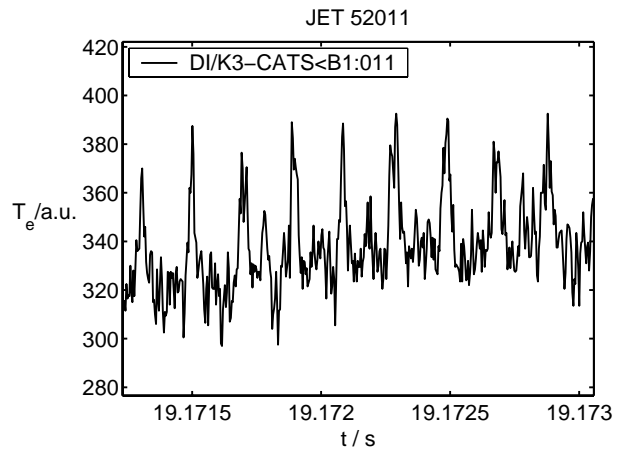
Figure 3: ECE signal at R = 3.84 m.
