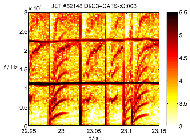
Figure 1: Magnetic spectrogram with palm tree modes in JET discharge 52148.
