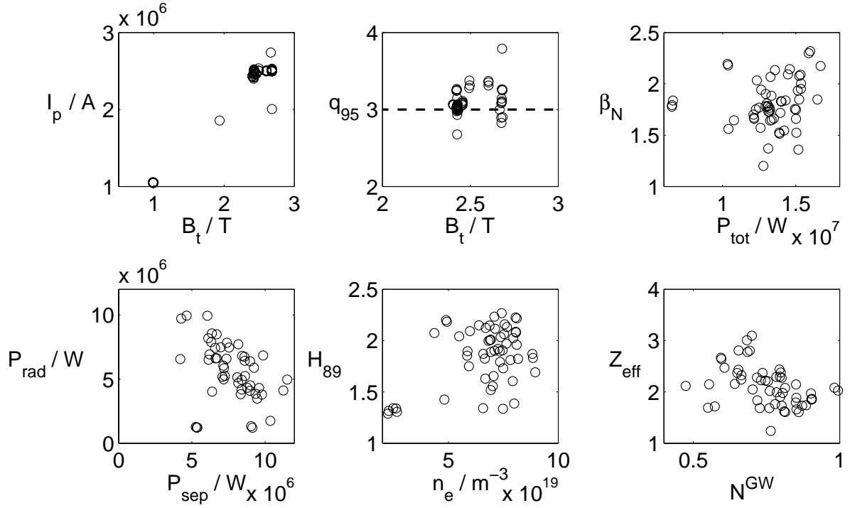
Figure 4: Overview on global plasma parameters where palm tree modes have been observed.
