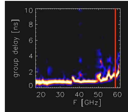
Fig. 2 – Example of group delay spectrogram slice (#19821)
