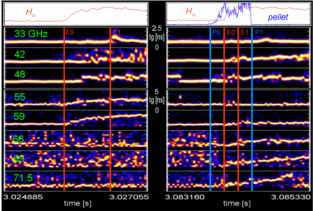
Fig. 5 – Temporal evolution of the GDSS for the intrinsic (left) and triggered (right) ELM at the HFS (#19821)
