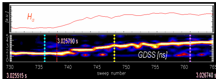
Fig. 3 – Temporal evolution of the HFS group delay spectrogram slice (GDSS) at 59 GHz (#19821)
