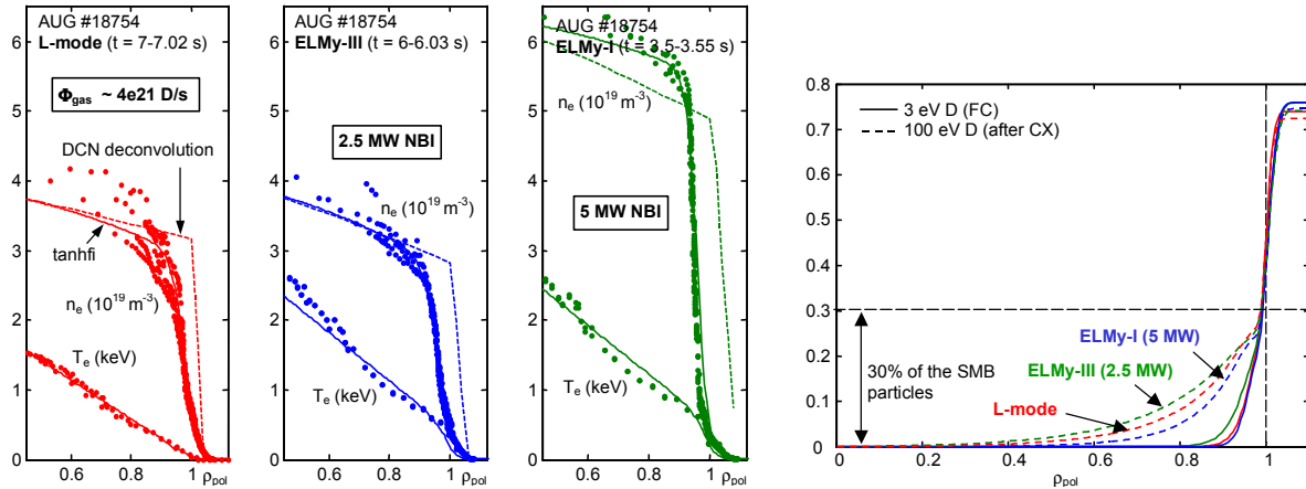
Figure 5. Edge electron temperature (ECE) and electron density profiles (O-mode reflectometry) in L-mode (0 MW NBI), ELM-III (2.5 MW NBI) and ELM-I phases (5 MW NBI) from #18754 and corresponding calculated integrated beam deposition as a function of the normalized poloidal flux radius.
