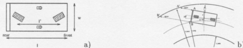
Figure 1: a) Schematic representation of a rhombic vehicle, showing its main dimensions; b) Vehicle alignment errors and clearance space ( space = \min\{AA', BB'\} ) in the TB gallery.
