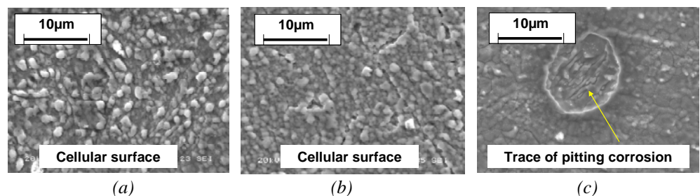
Fig.1 Surface image of specimens observed by SEM after immersion to (a) Li at 600°C, (b) Pb-17Li at 600°C, and (c) Flinak at 600°C
